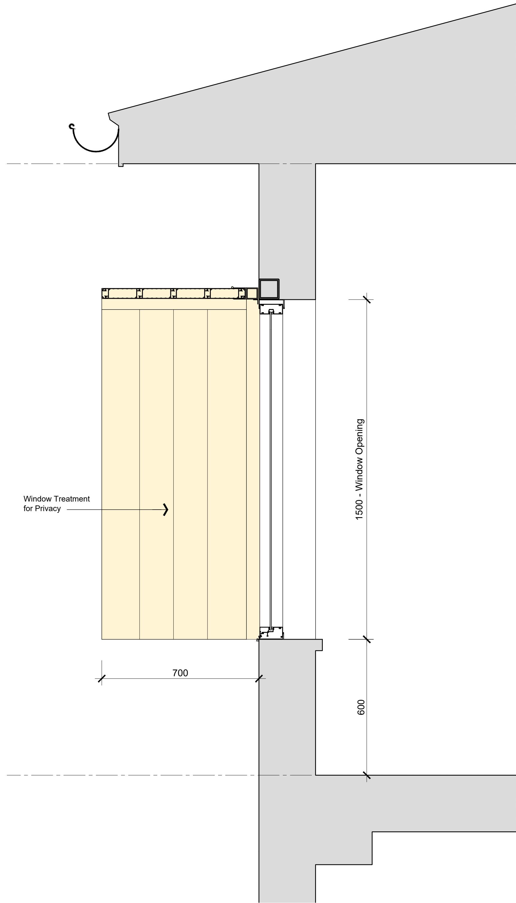
- Typical Detail of Window Treatment for Privacy Diagrammatic Only Scale 1:10
